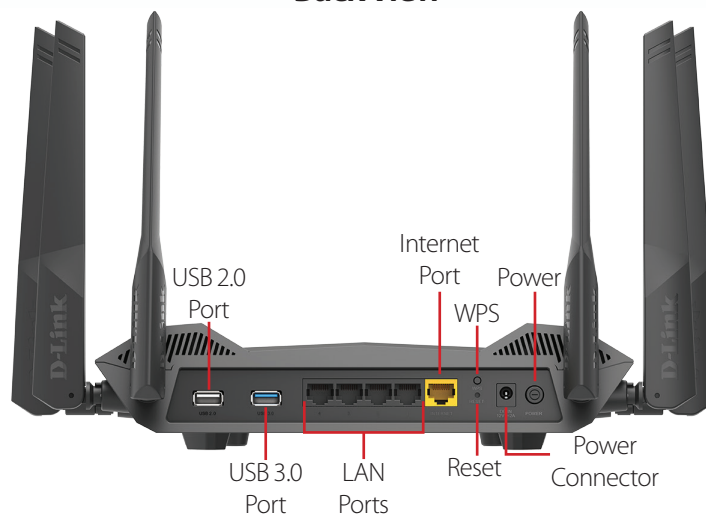
Back View
